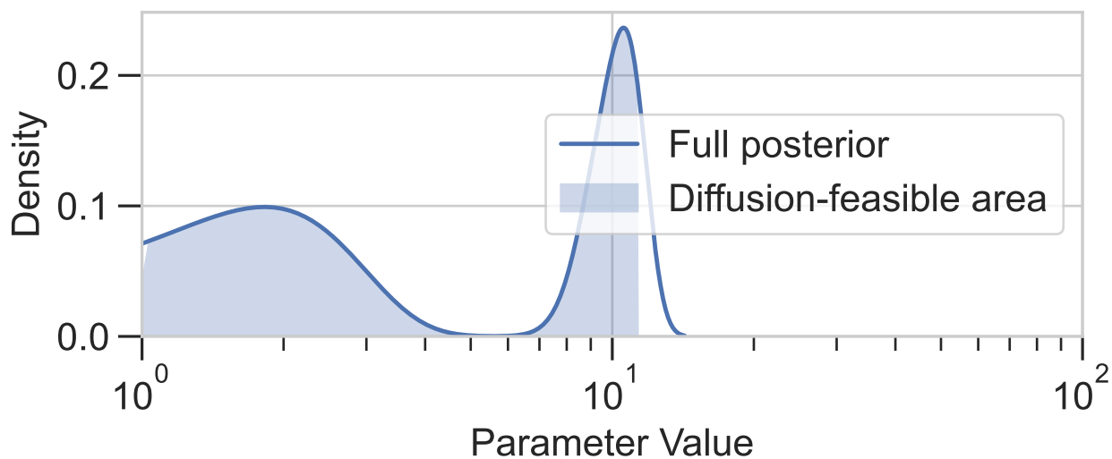
a1: Posterior with Diffusion-Feasible Area
