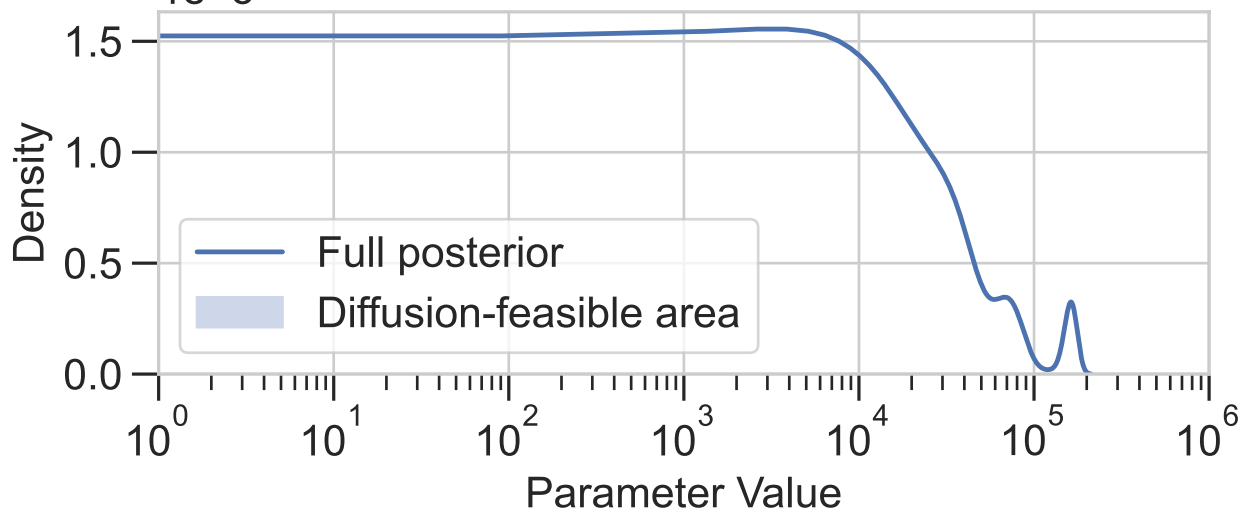
1e-5 c1: Posterior with Diffusion-Feasible Area
